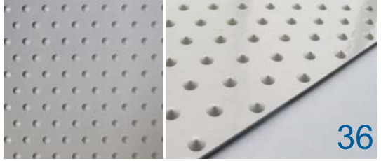
Name:Sharp nipple Thickness:1.4mm Property:- Application:Poultry,Sea food processing
